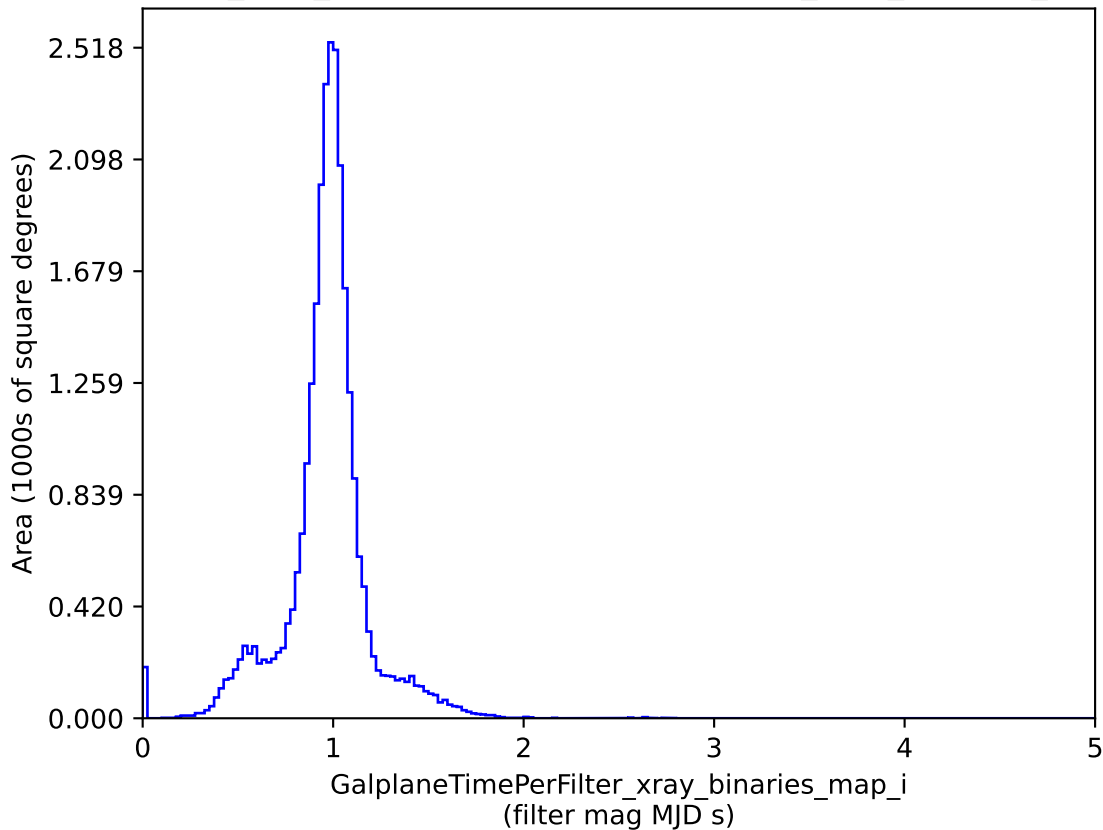
baseline_v2.0_10yrs : GalplaneTimePerFilter_xray_binaries_map_i
