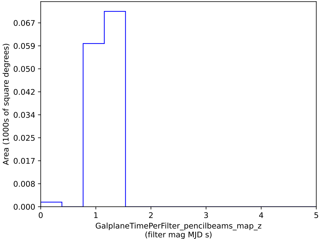
baseline_v2.0_10yrs : GalplaneTimePerFilter_pencilbeams_map_z
