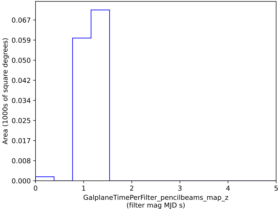
baseline_v2.0_10yrs : GalplaneTimePerFilter_pencilbeams_map_z
