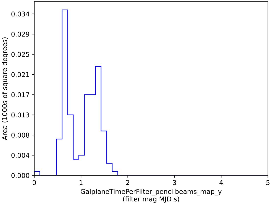
baseline_v2.0_10yrs : GalplaneTimePerFilter_pencilbeams_map_y
