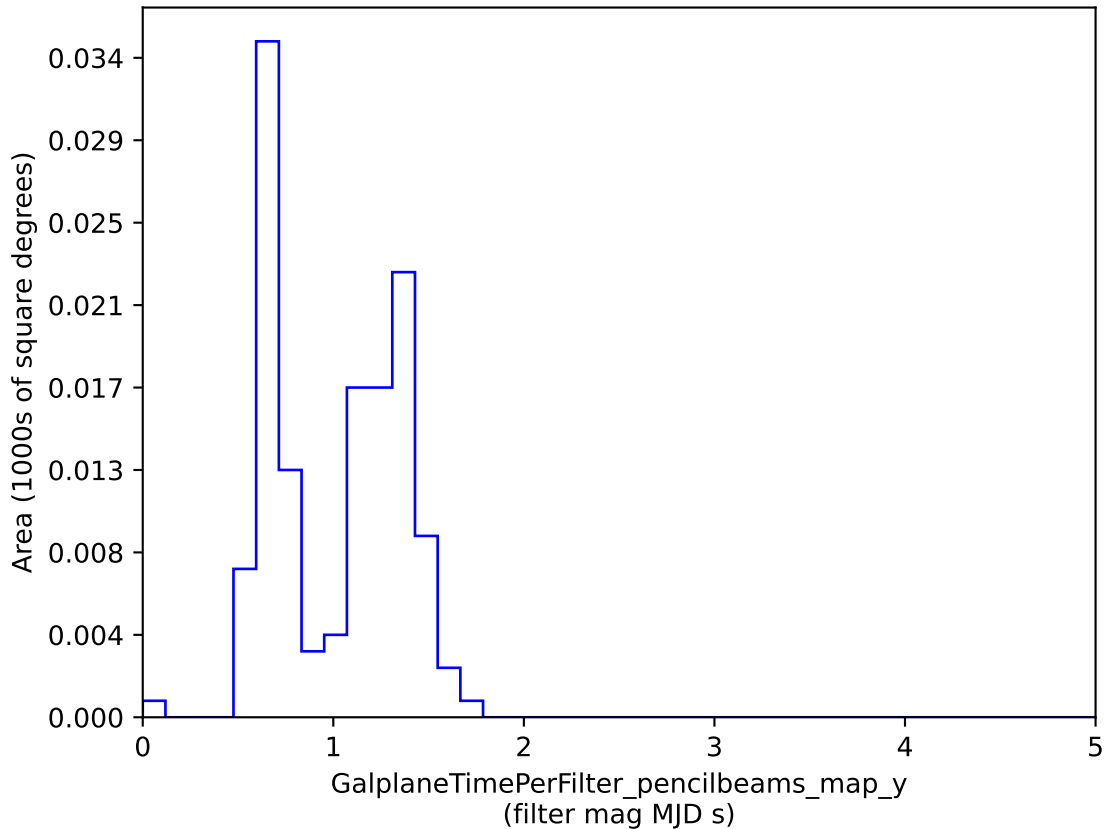
baseline_v2.0_10yrs : GalplaneTimePerFilter_pencilbeams_map_y
