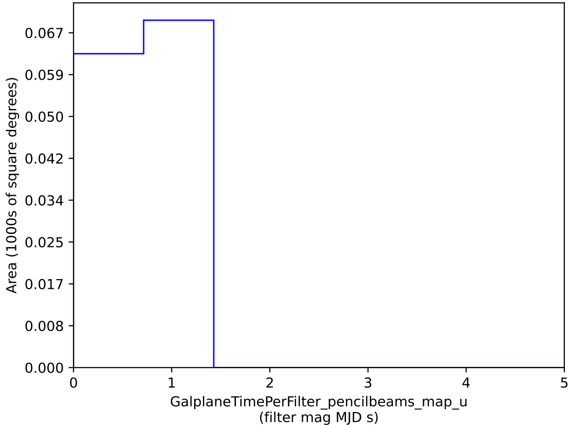
baseline_v2.0_10yrs : GalplaneTimePerFilter_pencilbeams_map_u
