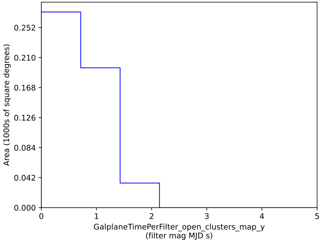
baseline_v2.0_10yrs : GalplaneTimePerFilter_open_clusters_map_y
