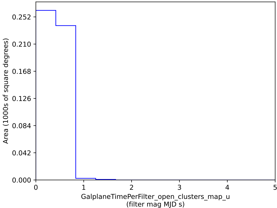
baseline_v2.0_10yrs : GalplaneTimePerFilter_open_clusters_map_u
