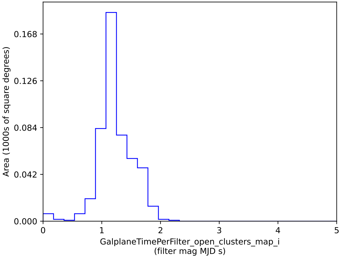
baseline_v2.0_10yrs : GalplaneTimePerFilter_open_clusters_map_i
