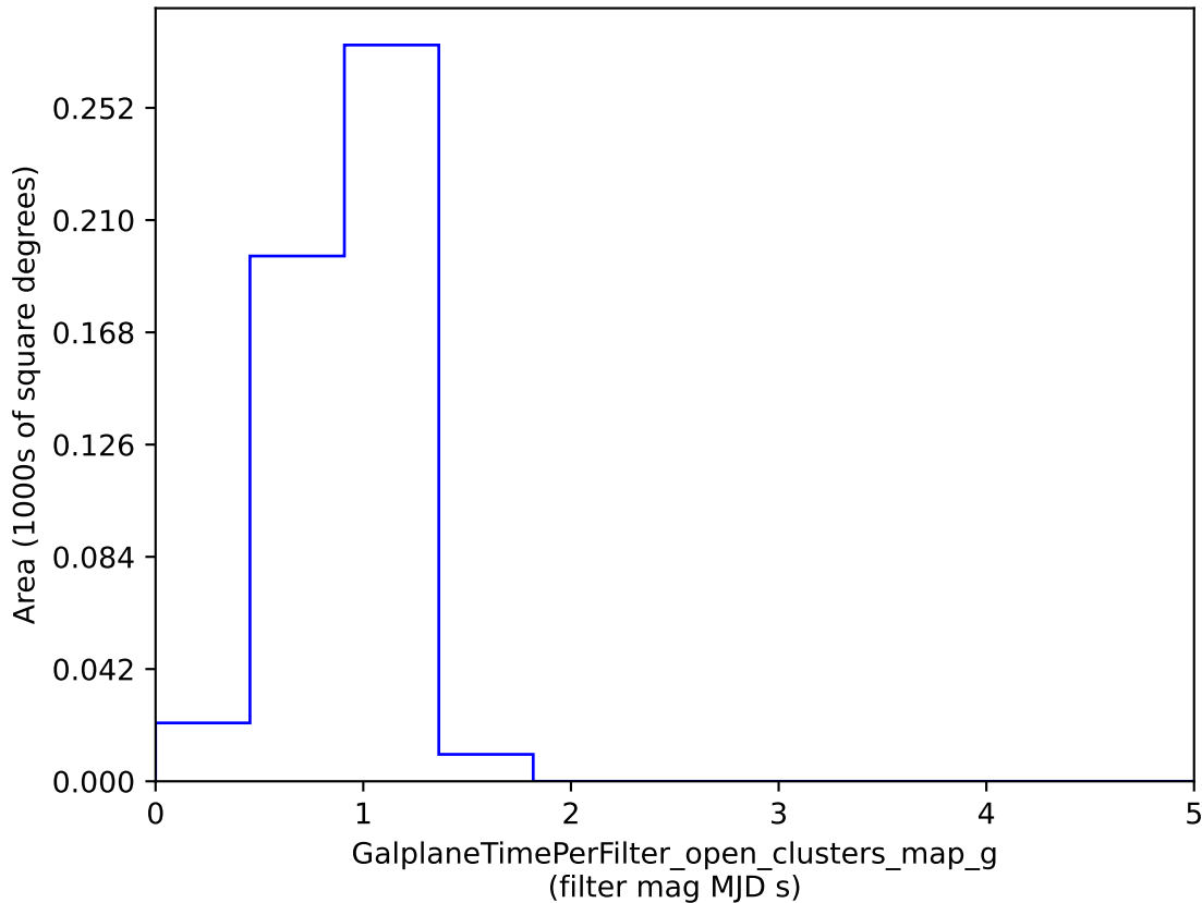
baseline_v2.0_10yrs : GalplaneTimePerFilter_open_clusters_map_g
