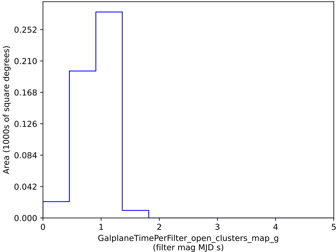
baseline_v2.0_10yrs : GalplaneTimePerFilter_open_clusters_map_g
