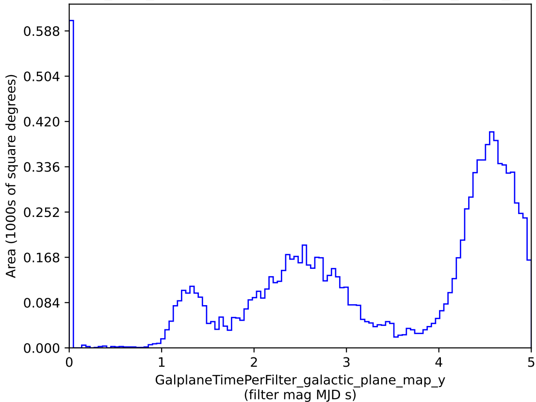
baseline_v2.0_10yrs : GalplaneTimePerFilter_galactic_plane_map_y
