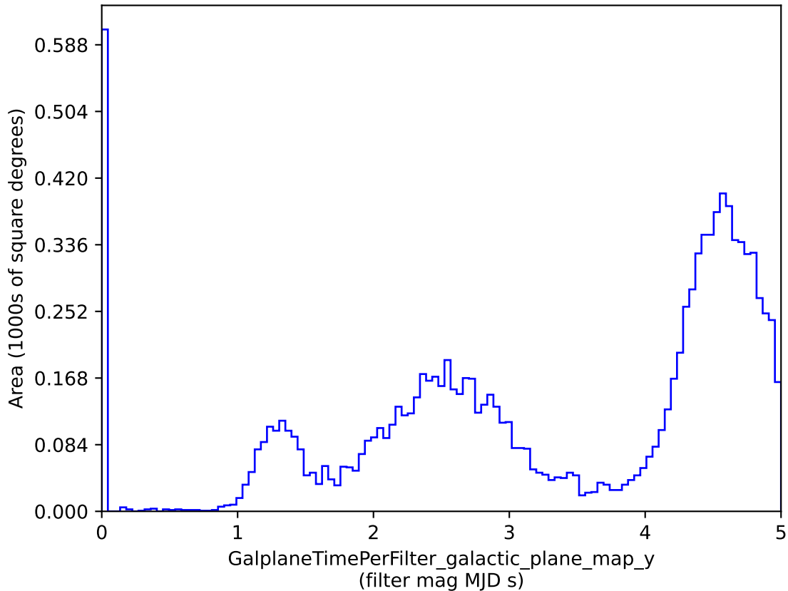
baseline_v2.0_10yrs : GalplaneTimePerFilter_galactic_plane_map_y
