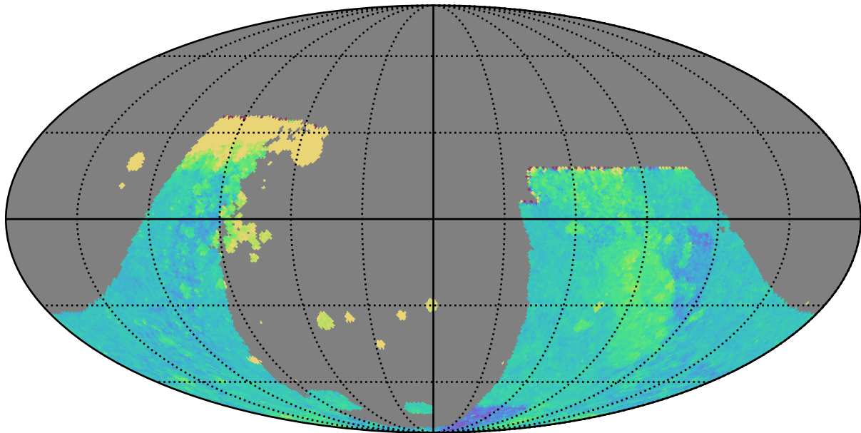
baseline_v2.0_10yrs : GalplaneTimePerFilter_combined_map_z
