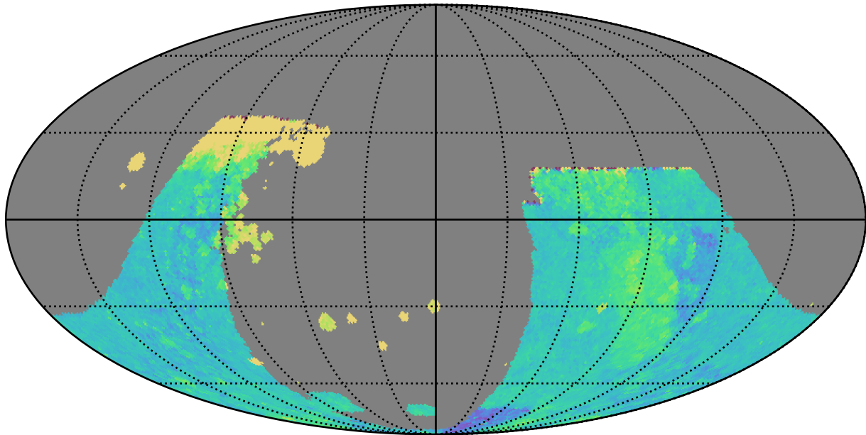
baseline_v2.0_10yrs : GalplaneTimePerFilter_combined_map_z
