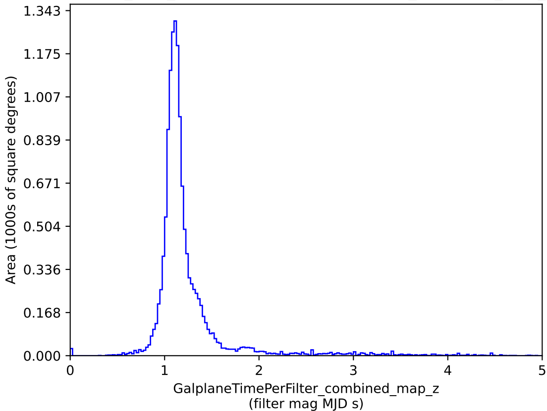
baseline_v2.0_10yrs : GalplaneTimePerFilter_combined_map_z
