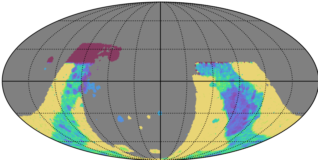
baseline_v2.0_10yrs : GalplaneTimePerFilter_combined_map_y
