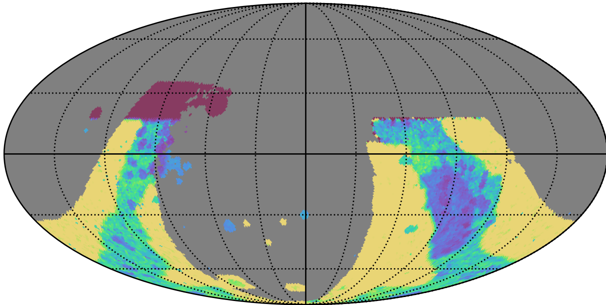
baseline_v2.0_10yrs : GalplaneTimePerFilter_combined_map_y
