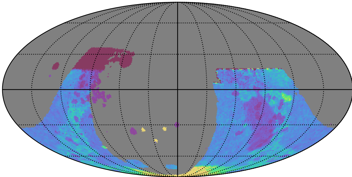
baseline_v2.0_10yrs : GalplaneTimePerFilter_combined_map_u
