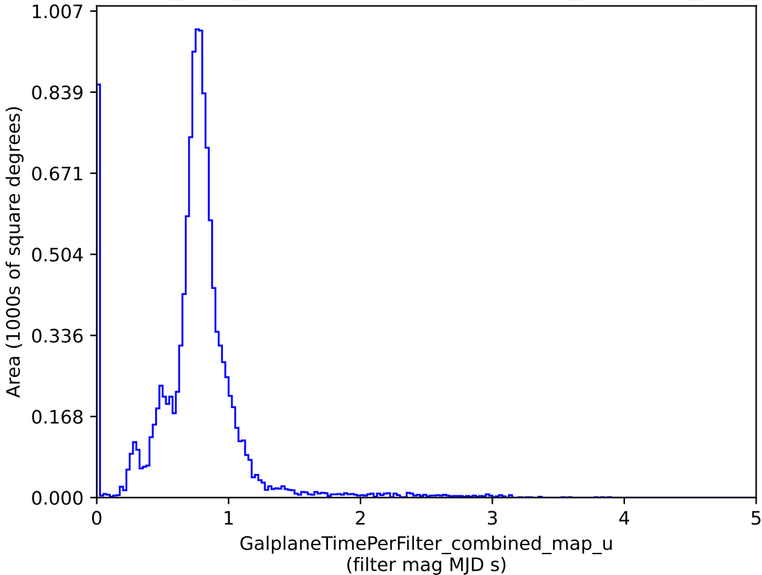
baseline_v2.0_10yrs : GalplaneTimePerFilter_combined_map_u
