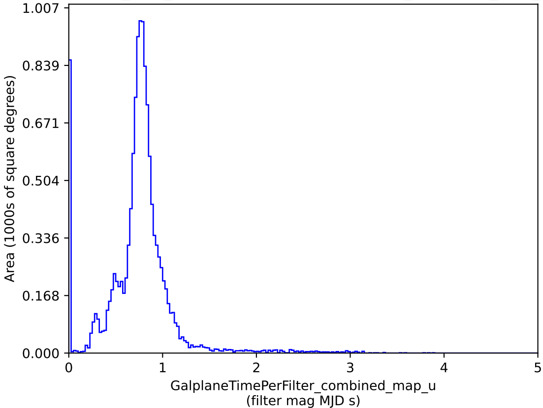
baseline_v2.0_10yrs : GalplaneTimePerFilter_combined_map_u
