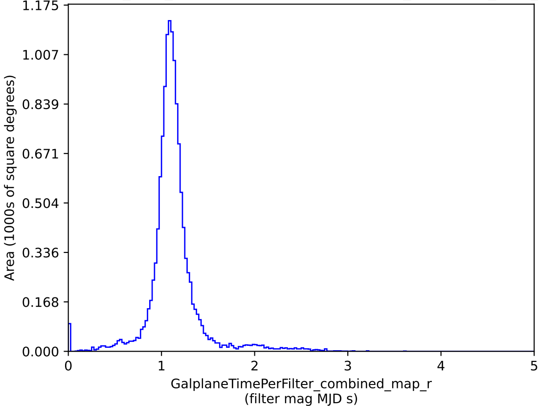
baseline_v2.0_10yrs : GalplaneTimePerFilter_combined_map_r
