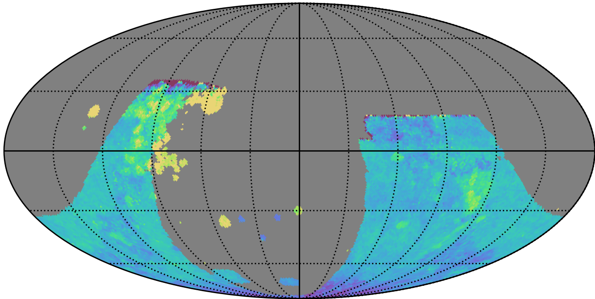
baseline_v2.0_10yrs : GalplaneTimePerFilter_combined_map_i
