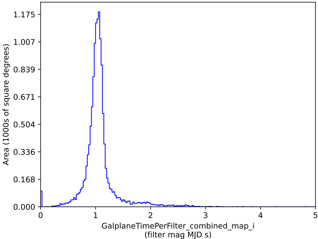
baseline_v2.0_10yrs : GalplaneTimePerFilter_combined_map_i
