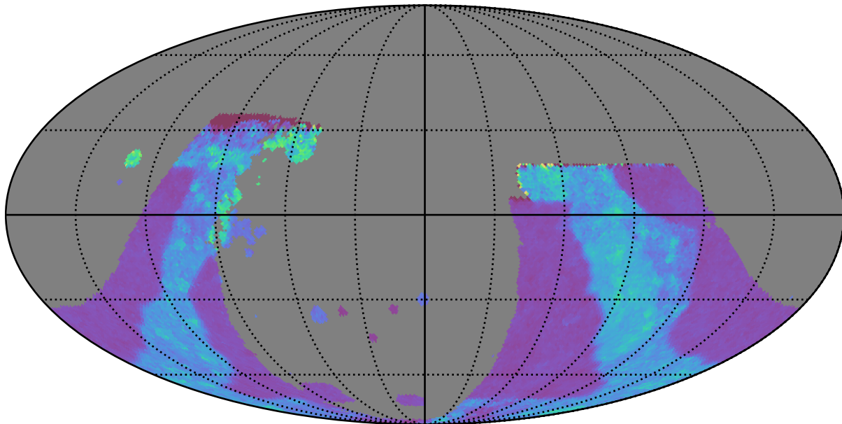
baseline_v2.0_10yrs : GalplaneTimePerFilter_combined_map_g
