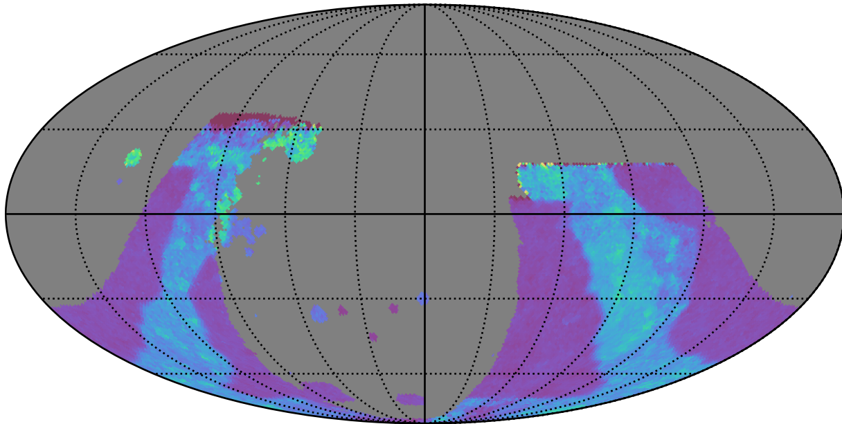
baseline_v2.0_10yrs : GalplaneTimePerFilter_combined_map_g
