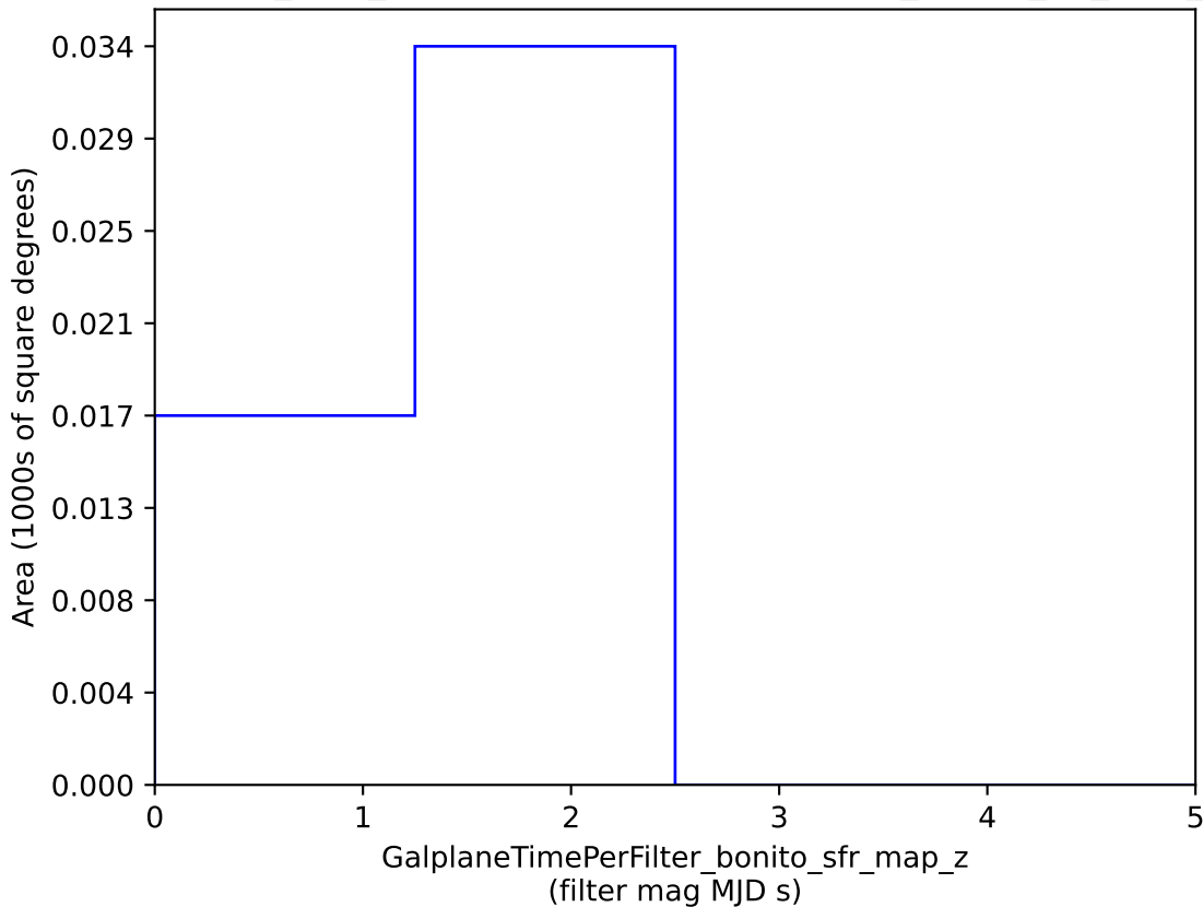
baseline_v2.0_10yrs : GalplaneTimePerFilter_bonito_sfr_map_z
