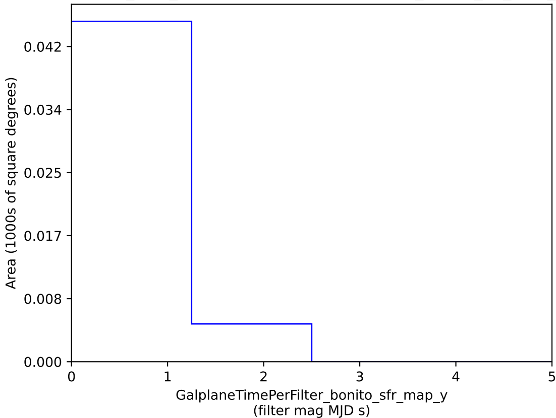
baseline_v2.0_10yrs : GalplaneTimePerFilter_bonito_sfr_map_y
