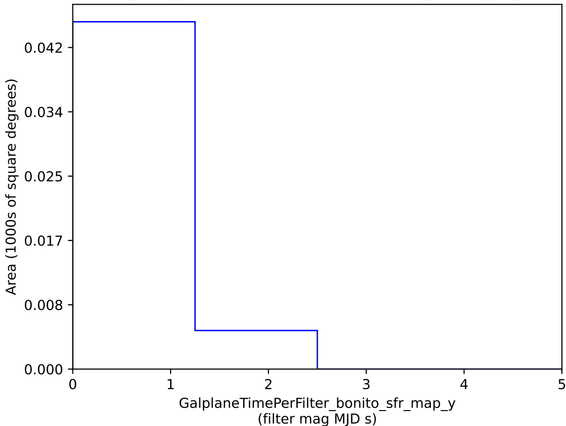
baseline_v2.0_10yrs : GalplaneTimePerFilter_bonito_sfr_map_y
