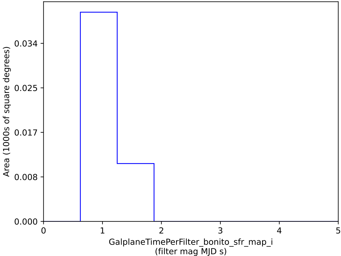
baseline_v2.0_10yrs : GalplaneTimePerFilter_bonito_sfr_map_i
