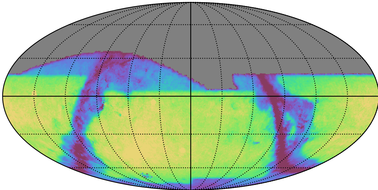
baseline_v2.0_10yrs z: GalaxyCountsMetricExtended
