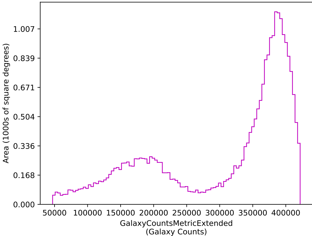
baseline_v2.0_10yrs z: GalaxyCountsMetricExtended
