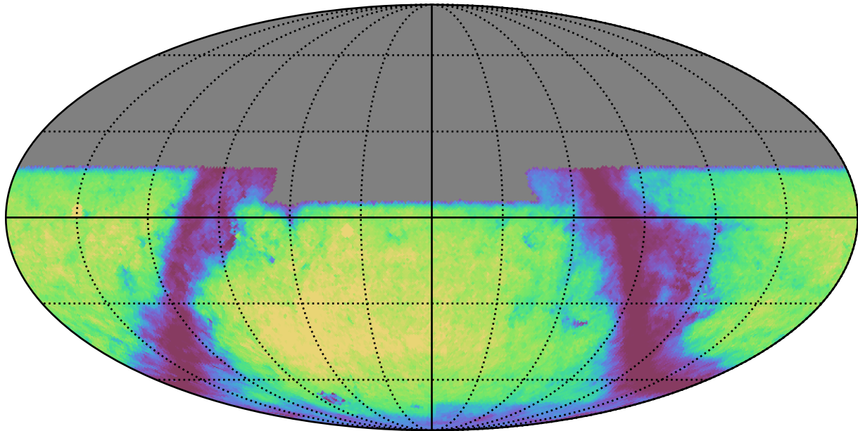
baseline_v2.0_10yrs u: GalaxyCountsMetricExtended
