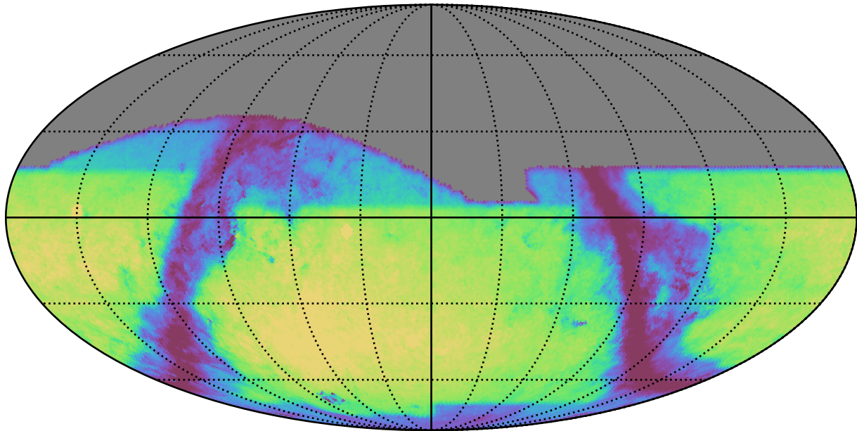
baseline_v2.0_10yrs r: GalaxyCountsMetricExtended
