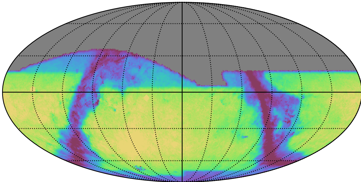
baseline_v2.0_10yrs i: GalaxyCountsMetricExtended
