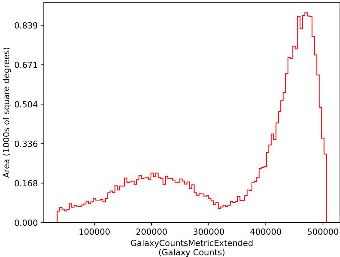
baseline_v2.0_10yrs i: GalaxyCountsMetricExtended
