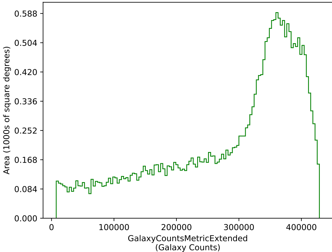
baseline_v2.0_10yrs g: GalaxyCountsMetricExtended
