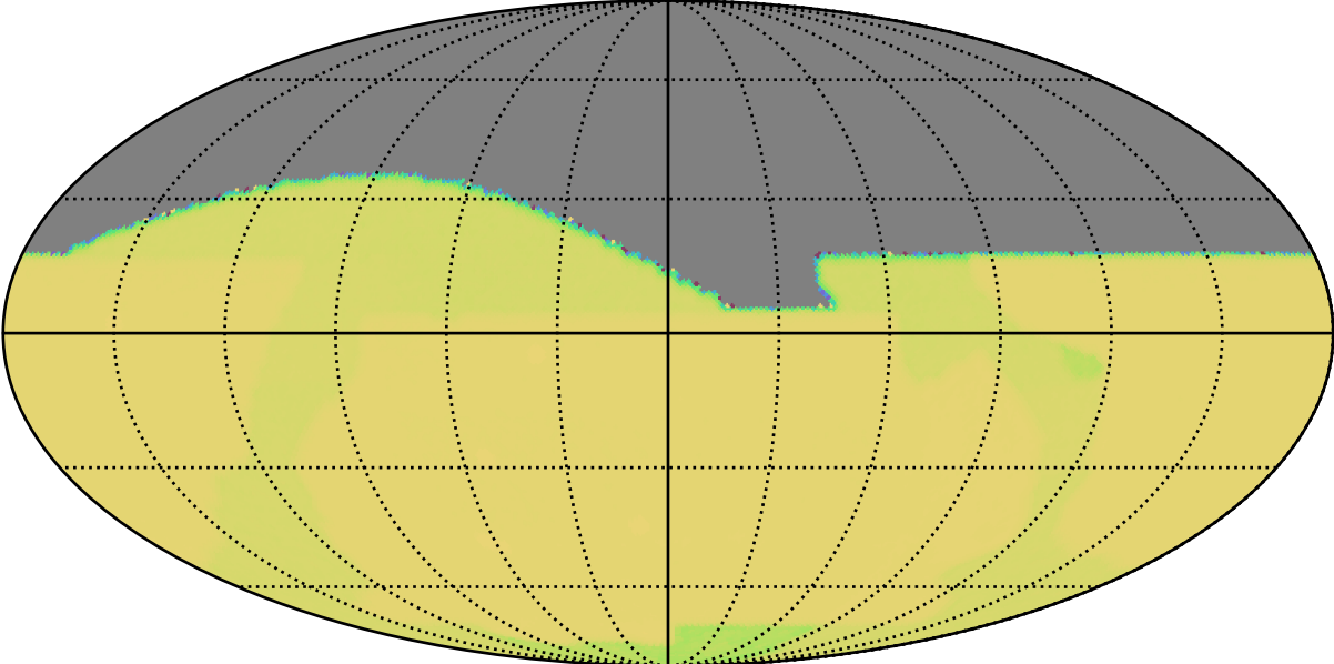
baseline_v2.0_10yrs : GalPlaneVisitIntervalsTimescales_xray_binaries_map_Tau_73_0
