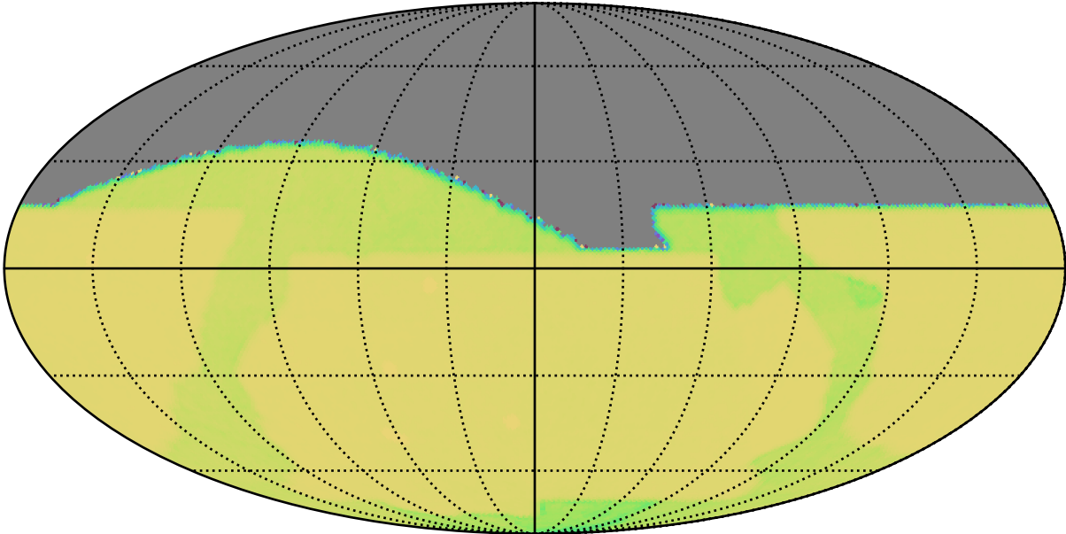
baseline_v2.0_10yrs : GalPlaneVisitIntervalsTimescales_xray_binaries_map_Tau_20_0
