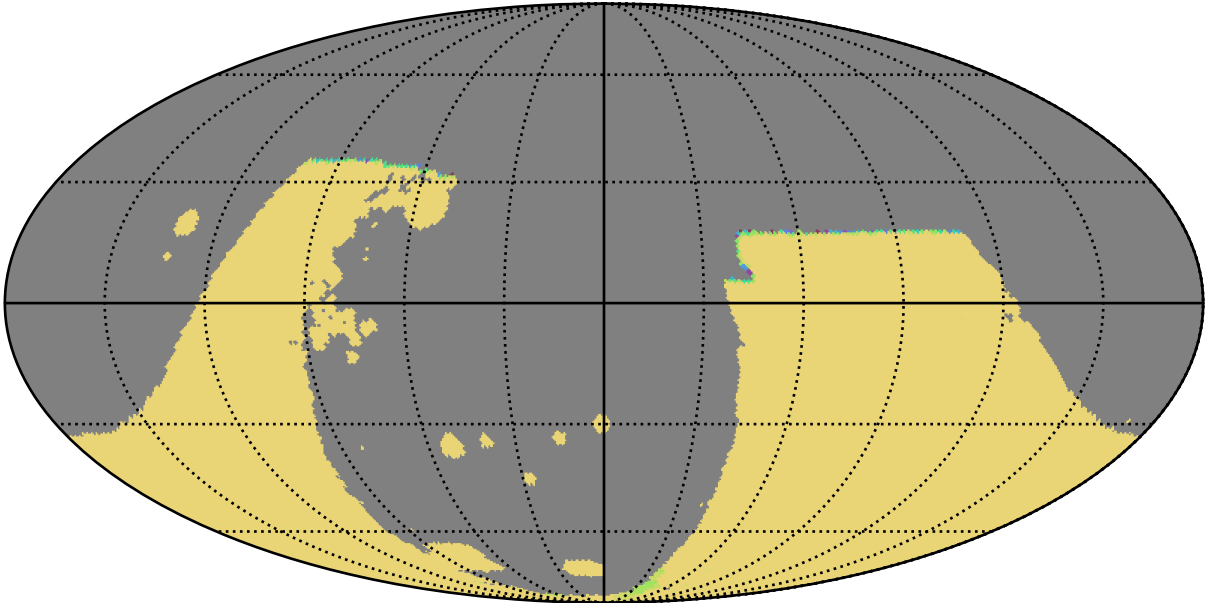
baseline_v2.0_10yrs : GalPlaneSeasonGapsTimescales_combined_map_Tau_365_0
