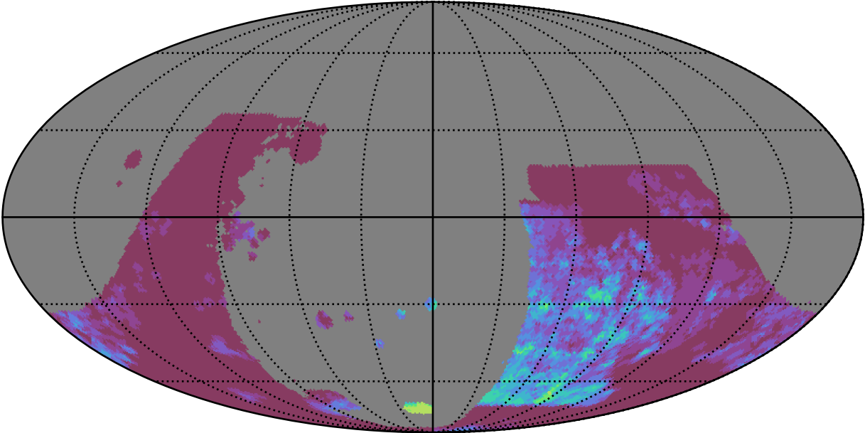
baseline_v2.0_10yrs : GalPlaneSeasonGapsTimescales_combined_map_Tau_25_0
