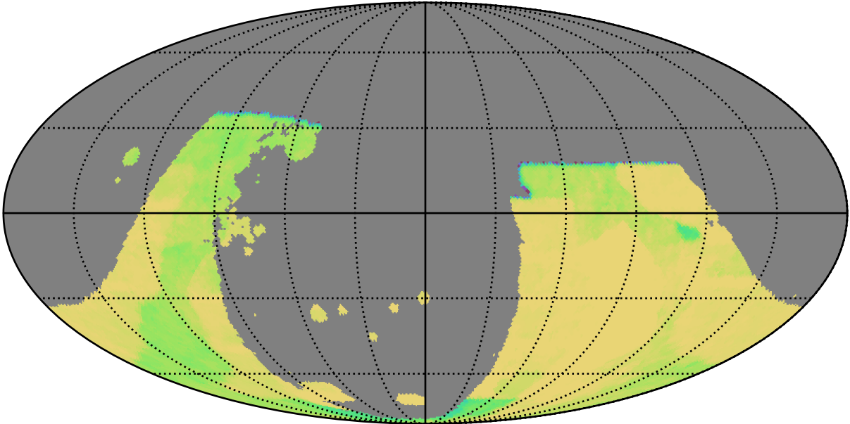
baseline_v2.0_10yrs : GalPlaneSeasonGapsTimescales_combined_map_Tau_232_5
