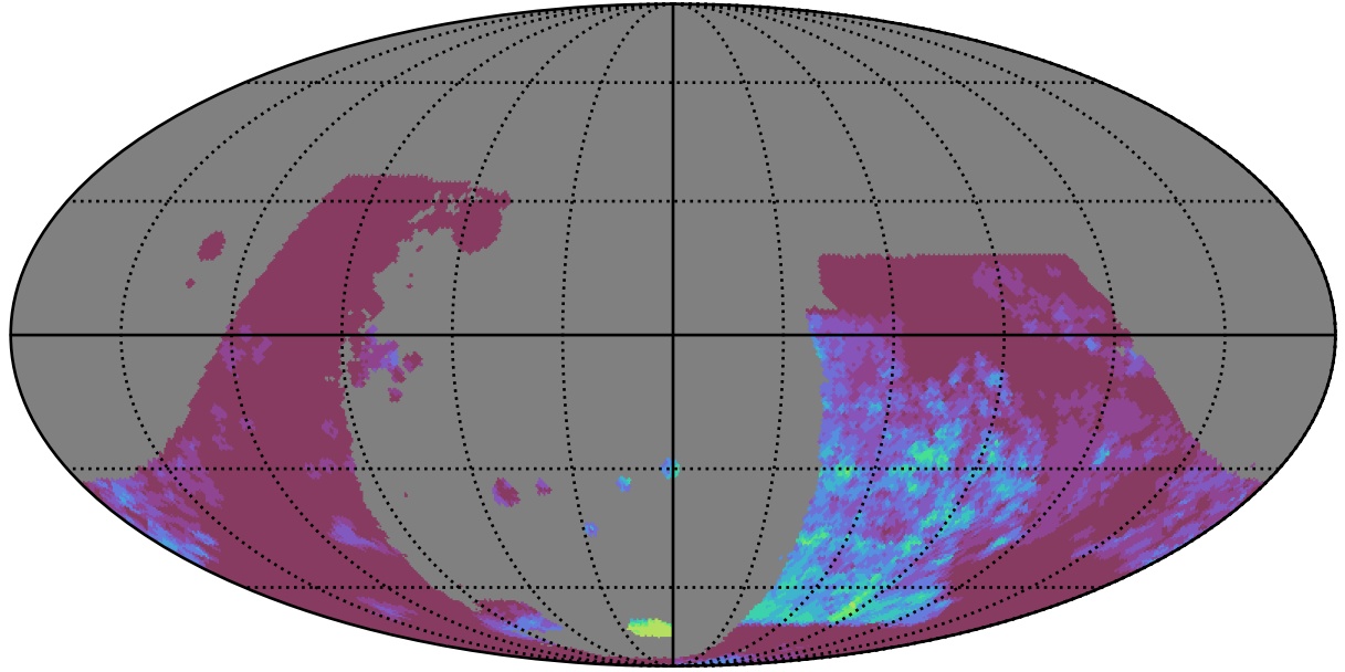
baseline_v2.0_10yrs : GalPlaneSeasonGapsTimescales_combined_map_Tau_10_0
