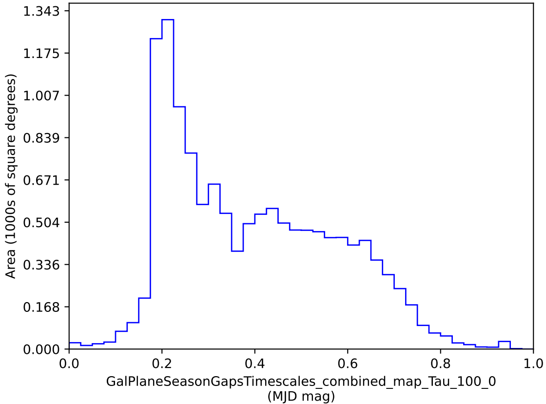
baseline_v2.0_10yrs : GalPlaneSeasonGapsTimescales_combined_map_Tau_100_0
