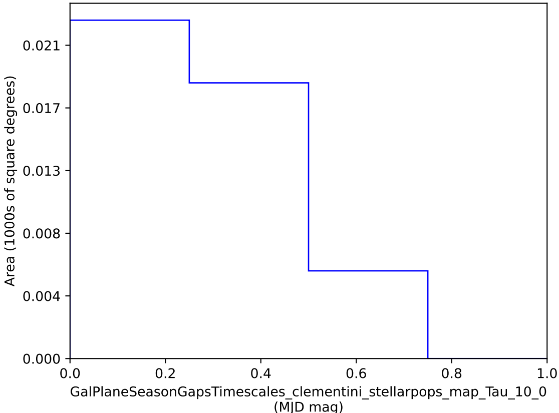
baseline_v2.0_10yrs : GalPlaneSeasonGapsTimescales_clementini_stellarpops_map_Tau_10_0
