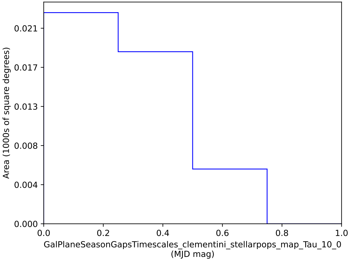
baseline_v2.0_10yrs : GalPlaneSeasonGapsTimescales_clementini_stellarpops_map_Tau_10_0
