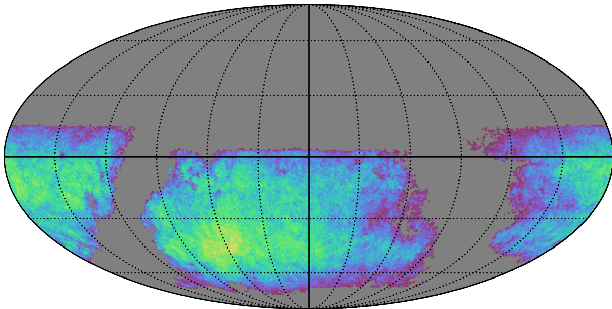
baseline_v2.0_10yrs i band non-DD year 9: ExgalM5WithCuts
