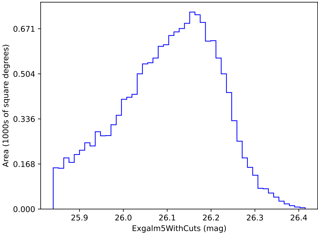
baseline_v2.0_10yrs i band non-DD year 9: ExgalM5WithCuts
