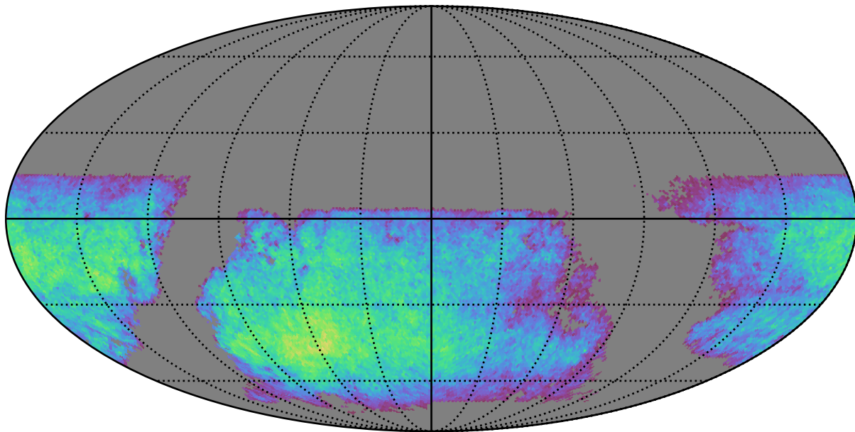
baseline_v2.0_10yrs i band non-DD year 8: ExgalM5WithCuts
