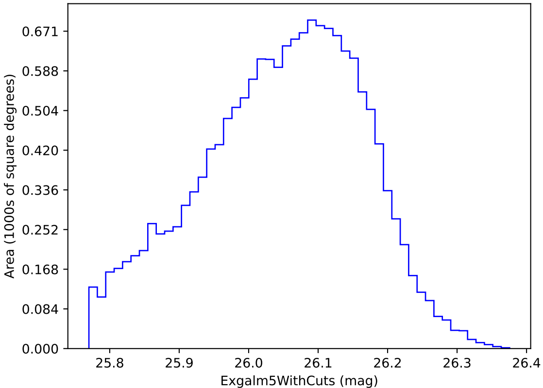
baseline_v2.0_10yrs i band non-DD year 8: ExgalM5WithCuts
