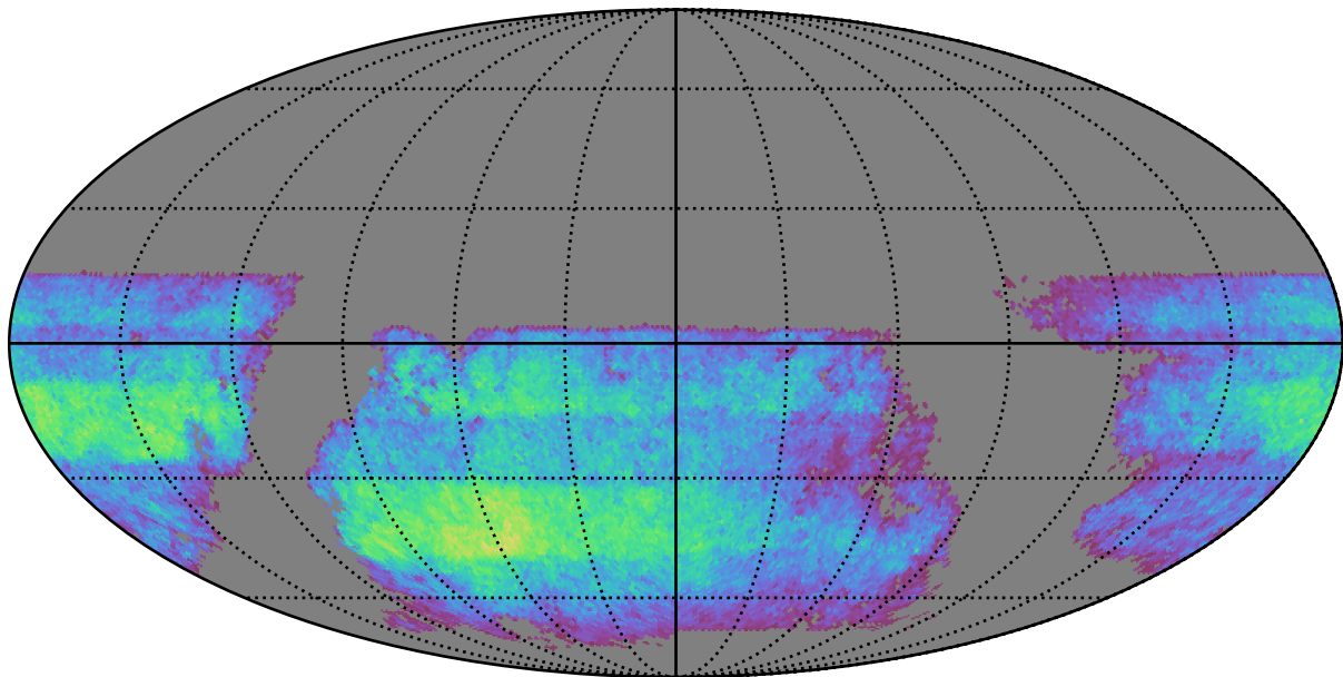
baseline_v2.0_10yrs i band non-DD year 7: ExgalM5WithCuts
