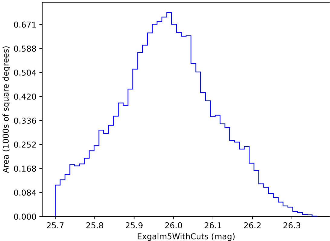
baseline_v2.0_10yrs i band non-DD year 7: ExgalM5WithCuts
