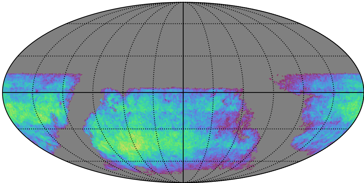
baseline_v2.0_10yrs i band non-DD year 6: ExgalM5WithCuts
