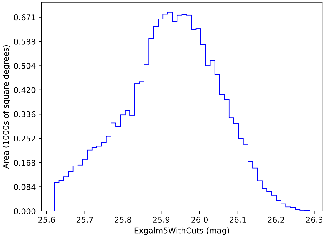
baseline_v2.0_10yrs i band non-DD year 6: ExgalM5WithCuts
