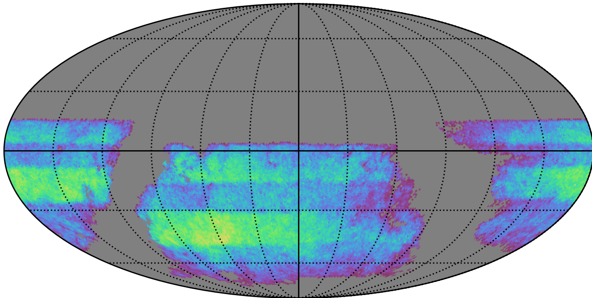
baseline_v2.0_10yrs i band non-DD year 5: ExgalM5WithCuts
