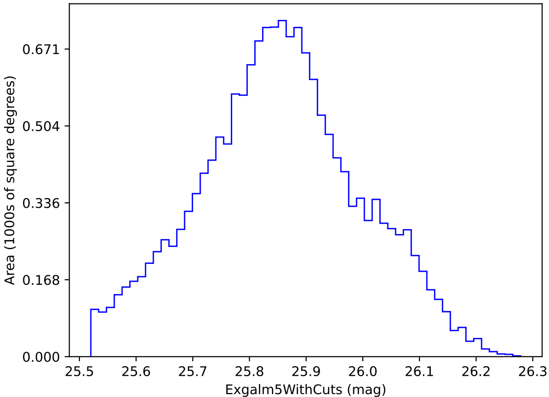
baseline_v2.0_10yrs i band non-DD year 5: ExgalM5WithCuts
