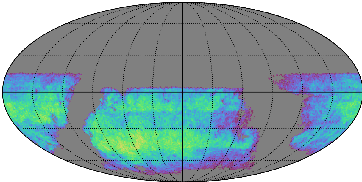
baseline_v2.0_10yrs i band non-DD year 4: ExgalM5WithCuts
