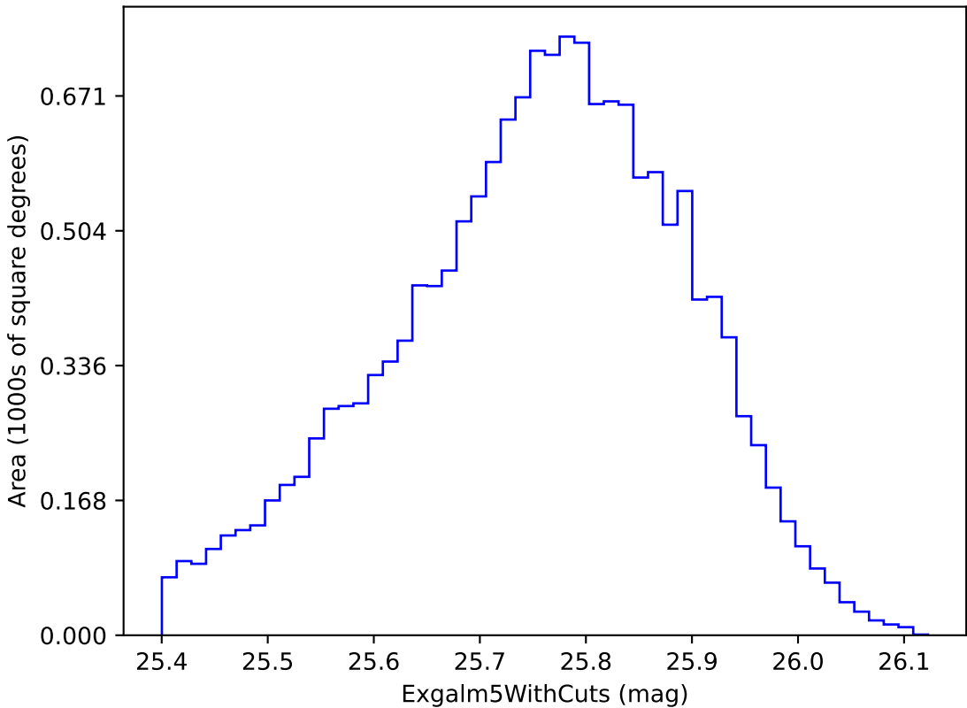
baseline_v2.0_10yrs i band non-DD year 4: ExgalM5WithCuts
