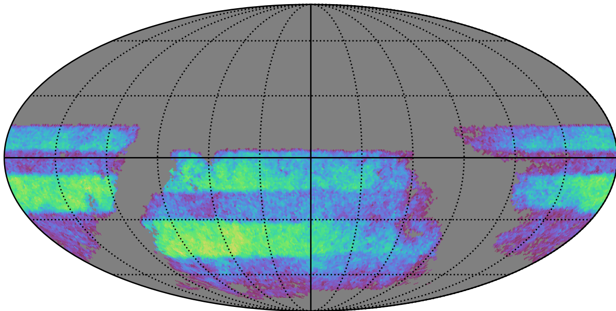
baseline_v2.0_10yrs i band non-DD year 3: ExgalM5WithCuts
