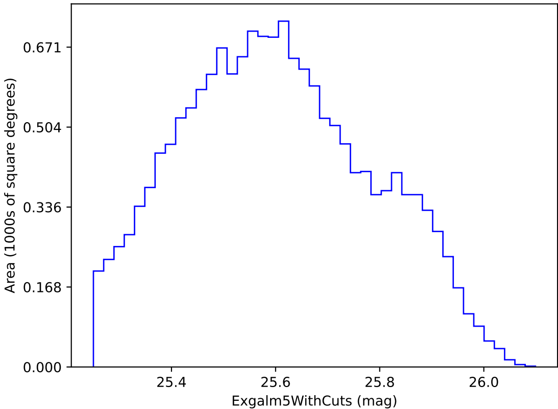
baseline_v2.0_10yrs i band non-DD year 3: ExgalM5WithCuts
